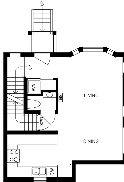
MAIN FLOOR 552 sq. ft.
