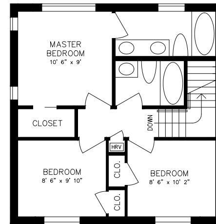
UPPER FLOOR 565 sq. ft.
