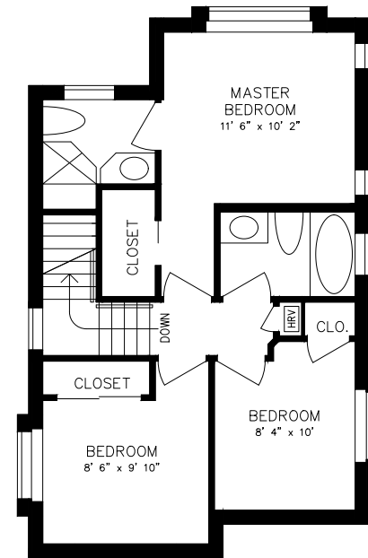
UPPER FLOOR 597 sq. ft.
